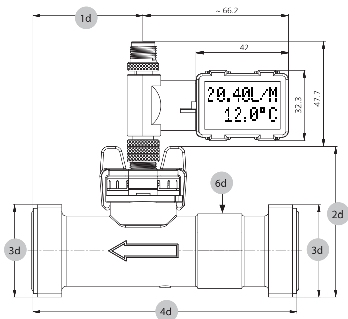
Dimension diagram DN 6, 8, 10, 15, 20, 25
