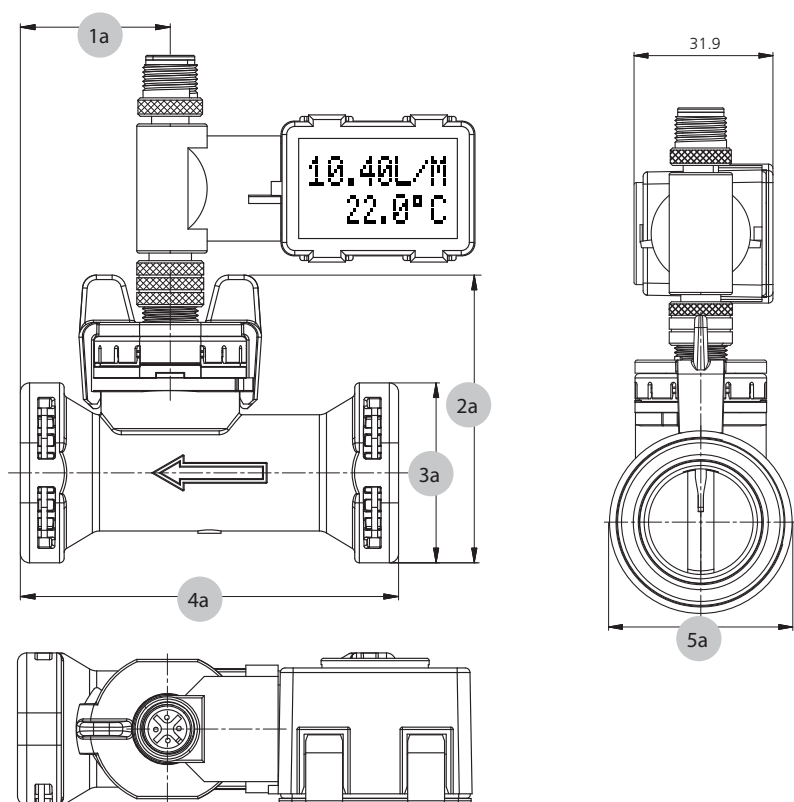
Dimension diagram DN 8, 10, 15, 20
