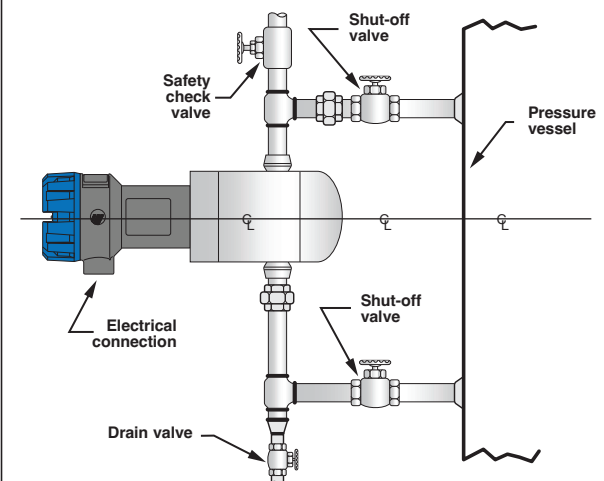
Typical piping arrangement
