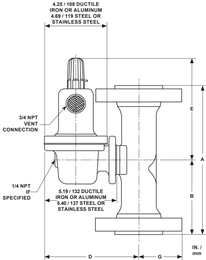
Figure 17. Flanged Dimensions
