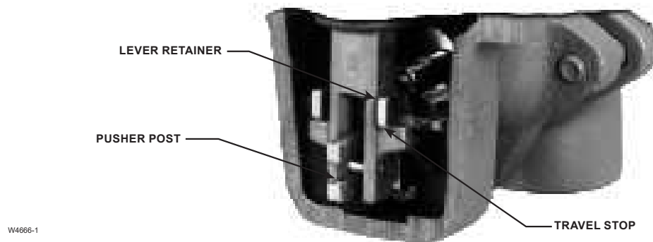
Figure 10. Internal Relief Construction Feature
