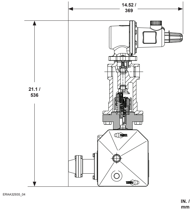
Figure 18. Type OSX Slam-Shut Valve Dimensions
