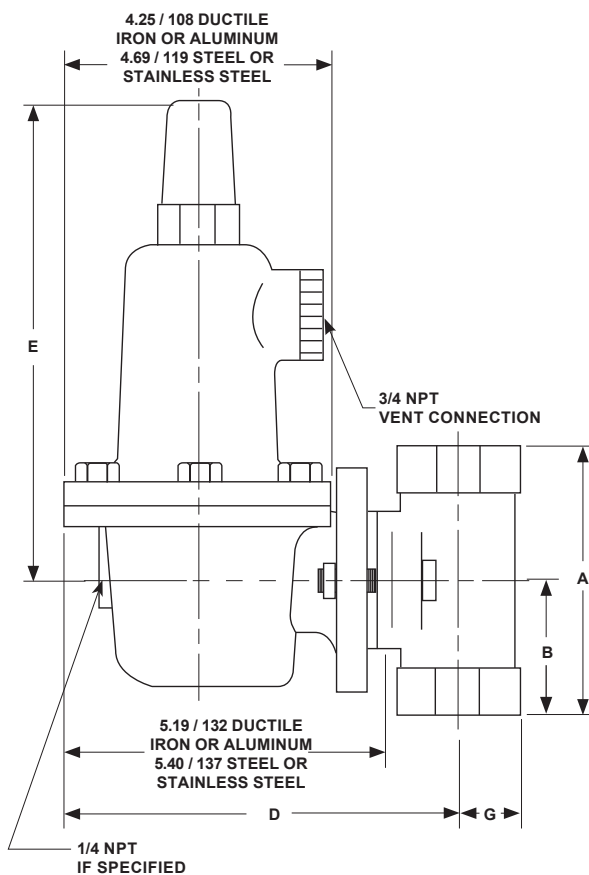
Figure 15. NPT Dimensions
